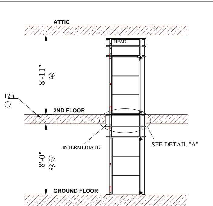
VIEW "A-A"
